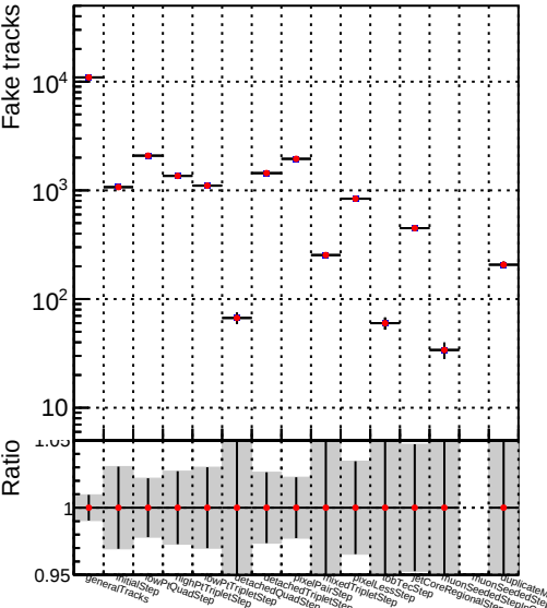
Number —●— DQM_CKF_TT_baseT125_noSel
