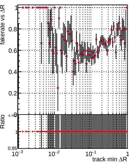
Fake rate vs \Delta R(\text{track, jet}) Legend: \Delta R(\text{track, jet}) (black line) \Delta R(\text{track, jet}) (red line)
