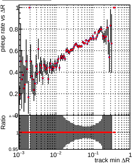
Legend: \Delta R CKF TT base noSel (grey line with error bars) \Delta R CKF TT baseT125 noSel (red line with error bars)
