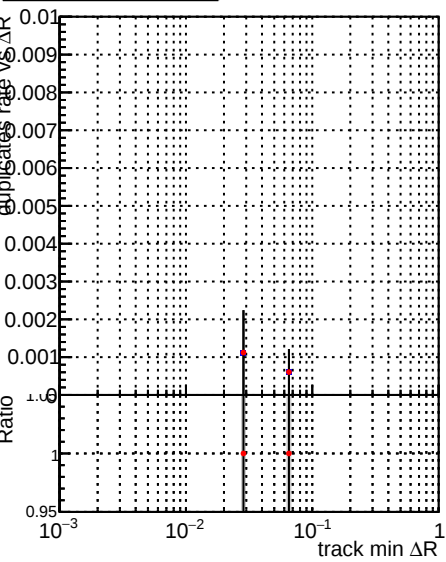
Legend: \Delta R CKF TT base noSel (grey line with error bars) \Delta R CKF TT baseT125 noSel (red line with error bars)
