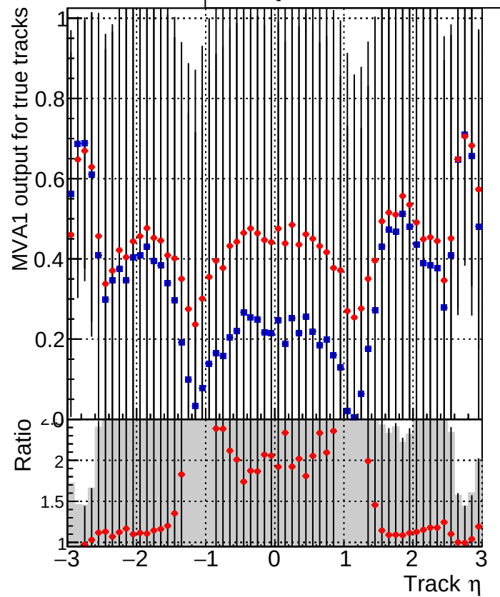
MVA1 of associated tracks (recoToSim) vs. track \eta ■ DQM_CKF_TT_base_noSel ◆ DQM_CKF_TT_baseT125_noSel
