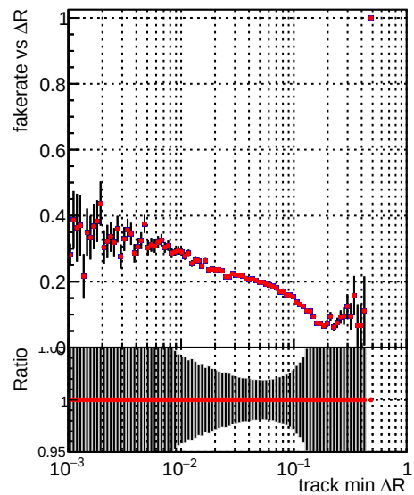
—•— DQM_CKF_TT_base_noSel —•— DQM_CKF_TT_baseT125_noSel
