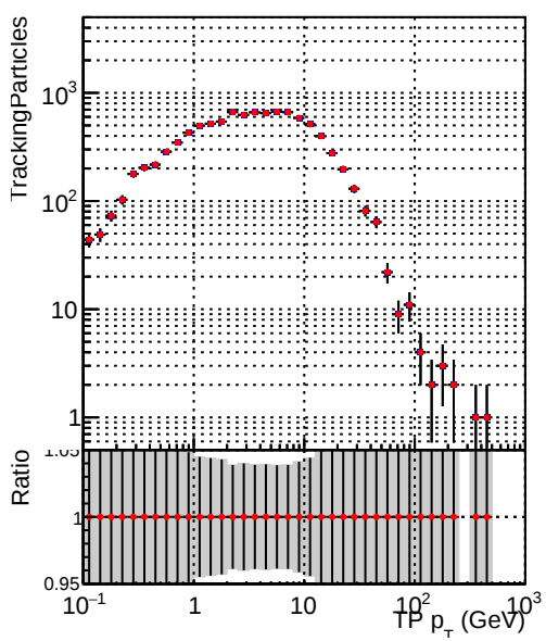
—•— DQM_CKF_TT_base_noSel —•— DQM_CKF_TT_baseT125_noSel
