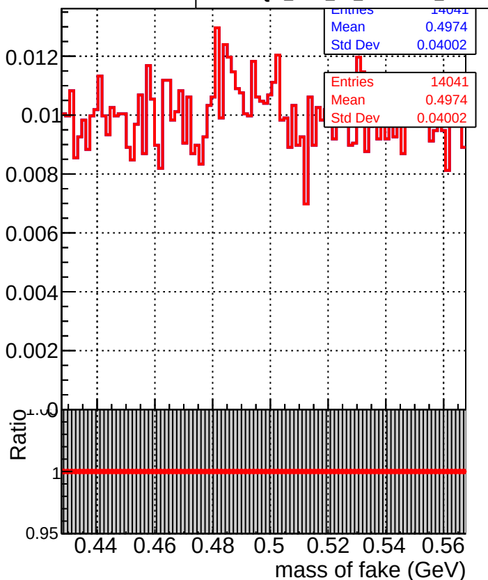
Mass of fake K0S
