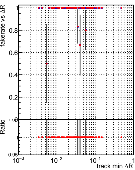
Fake rate vs \Delta R(\text{track, jet}) —●— DQM_CKF_TT_base_noSel —●— DQM_CKF_TT_baseT125_noSel
