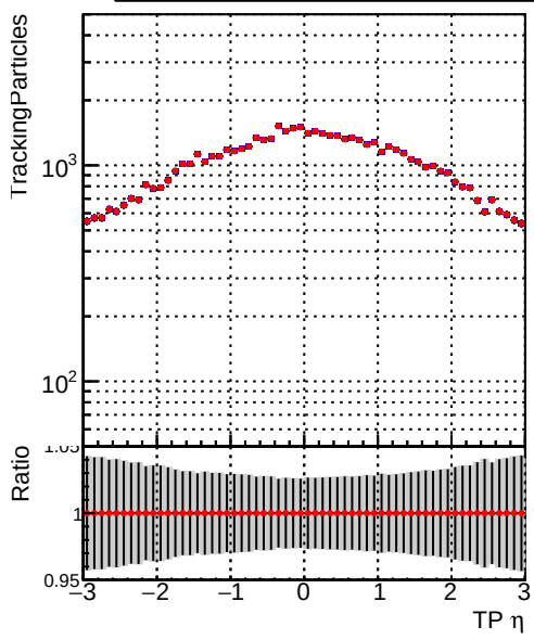
N of simulated tracks vs eta Legend: DQM_CKF_TT_base_noSel (blue line with dots), DQM_CKF_TT_baseT125_noSel (red line with dots)
