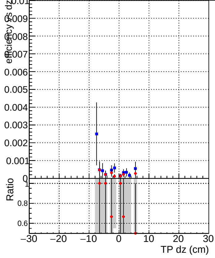
Efficiency vs Dz Legend: DQM_mkFit_TTbase (blue square) DQM_mkFit_TT_retrainOldFiles125 (red circle)
