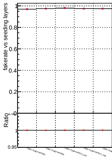
Fake rate vs. —•— DQM_mkFit_TTbase —•— DQM_mkFit_TT_retrainOldFiles125
