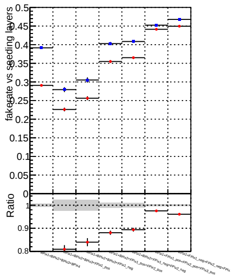
Fake rate vs. Legend: DQM_mkFit_TTbase (Blue circles) DQM_mkFit_TT_retrainOldFiles125 (Red circles)
