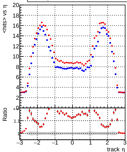
mean hits Legend: DQM_mkFit_TTbase (blue line), DQM_mkFit_TT_retrainOldFiles125 (red line)
