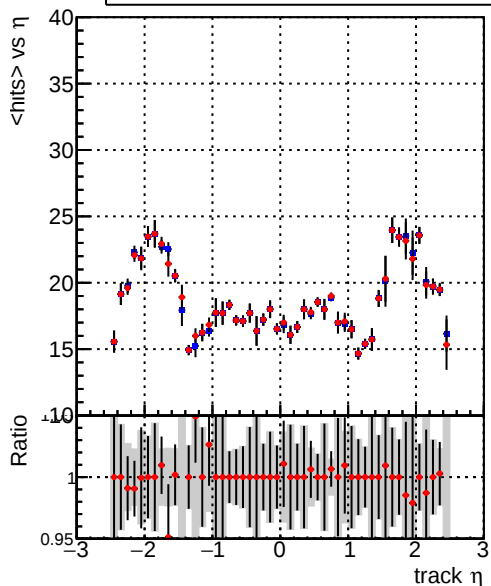
mean hits vs \eta Legend: DQM_mkFit_TTbase (blue line), DQM_mkFit_TT_retrainOldFiles125 (red line)
