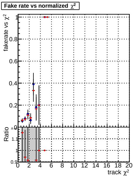
Fake rate vs. —•— DQM_mkFit_TTbase —•— DQM_mkFit_TT_retrainOldFiles125
