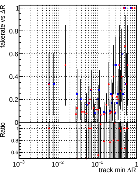
Fake rate vs \Delta R(\text{track, jet}) Legend: DQM_mkFit_TTbase (blue squares), DQM_mkFit_TT_retrainOldFiles125 (red circles)
