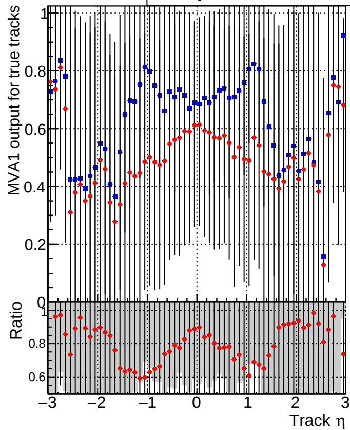
MVA1 of associated tracks (recoToSim) vs. Track \eta Legend: ■ DQM_mkFit_TTbase ● DQM_mkFit_TT_retrainOldFiles125
