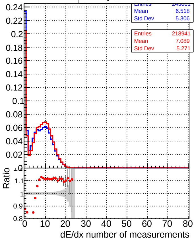
Legend: DQM_mkFit_TTbase (Blue line with squares) DQM_mkFit_TT_retrainOldFiles125 (Red line with circles)
