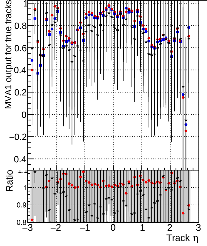
MVA1 of associated tracks (recoToSim) vs. track \eta Legend: DQM_CKF_TT_base_noSel (blue squares) DQM_CKF_TT_retrainOldFiles113_noSel (red diamonds) DQM_CKF_TT_retrainOldFiles125_noSel (black stars)
