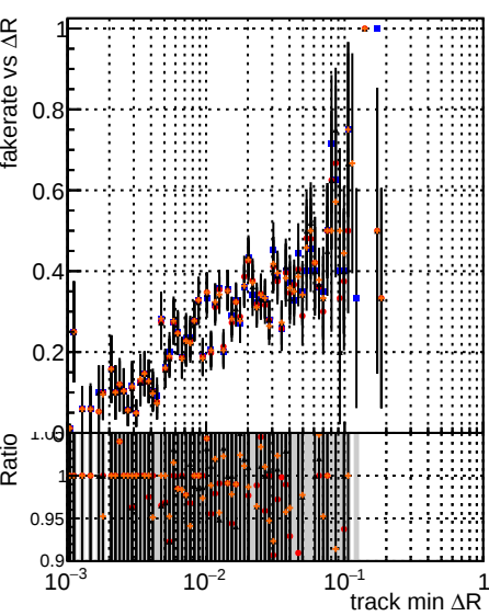
Fake rate vs \Delta R(\text{track, jet}) Legend: DOM mktFit Tbase retrainOldFiles125 DOM mktFit Tbase retrainNewFiles125 DOM mktFit Tbase retrainNewFiles125AndSQCD
