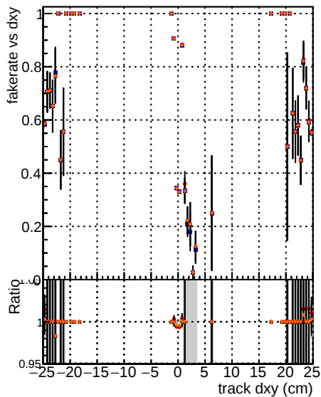
DQM mkt Fit Tbase DQM mkt Fit Tbase Fake rate vs d Duplicates Rate vs Dxy Pileup rate vs dxy
