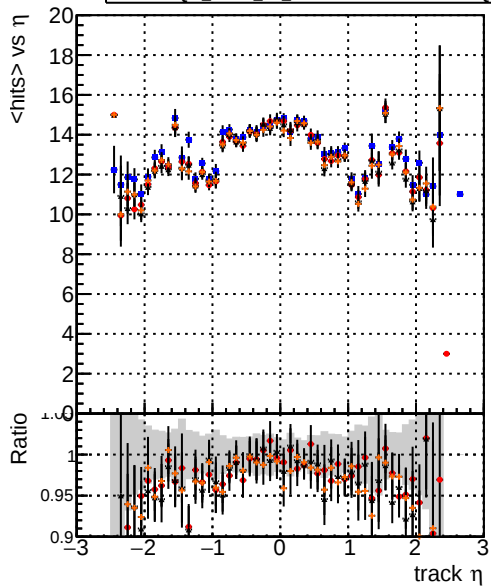
mean hit DOM_mkFit_TTbase DOM_mkFit_TT_retrainOldFiles125 DOM_mkFit_TT_retrainNewFiles125 DOM_mkFit_TT_retrainNewFiles125AndSQCD
