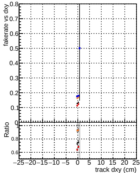
Legend: - Blue: BSM mkFit TTbase - Red: BSM mkFit TTbase OldFiles125 - Orange: BSM mkFit TTbase NewFiles125 - Black: BSM mkFit TTbase AndSQCD
