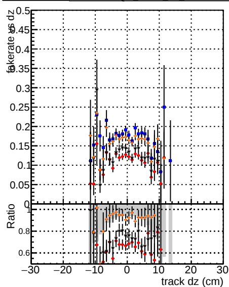
Legend: - Blue: BSM mkFit TTbase - Red: BSM mkFit TTbase OldFiles125 - Orange: BSM mkFit TTbase NewFiles125 - Black: BSM mkFit TTbase AndSQCD
