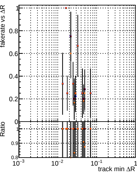
Fake rate vs \Delta R(\text{track, jet}) Legend: DOM mkFit Tbase (blue) DOM mkFit retrainOldFiles125 (red) DOM mkFit retrainNewFiles125 (orange) DOM mkFit retrainNewFiles125AndSQCD (grey)
