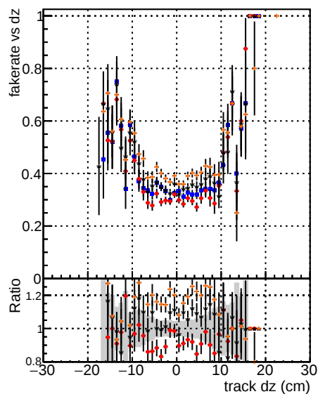
Fake rate vs dz Legend: BSM mktFit TTbase, BSM mktFit TTbase+OLDFiles125, BSM mktFit TTbase+NEWFiles125, AndSQCD
