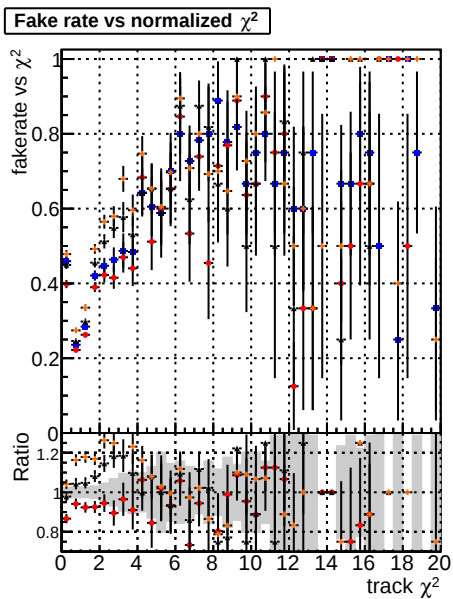
Fake rate vs. \chi^2 for BQM, mkFit, TTbase, and Ttbase. The legend indicates the methods used for the data points.
