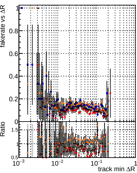
Fake rate vs \Delta R(\text{track, jet}) Legend: DOM mkFit (black) DOM mkFit + Tbase (blue) DOM mkFit + retrainOldFiles125 (red) DOM mkFit + retrainNewFiles125AndSQCD (orange)
