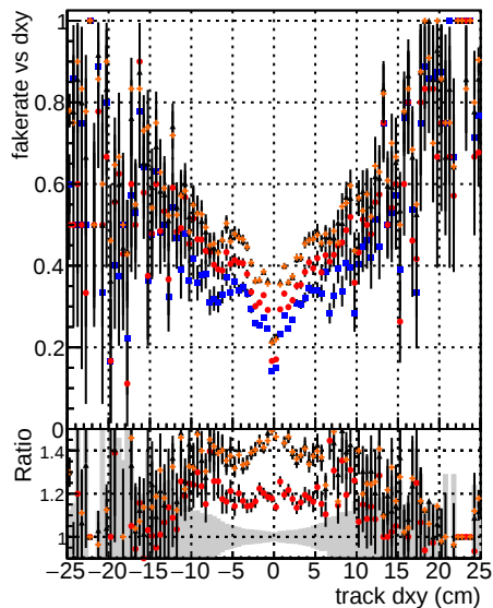
Legend: BQM mkt Fit TTbase TrainOldFiles125 TrainNewFiles125 AndSQCD
