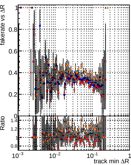
Fake rate vs \Delta R(\text{track, jet}) Legend: DOM (black) mktFit (blue) mktFit+base (red) retrainOldFiles125 (orange) retrainNewFiles125 (green) retrainNewFiles125AndSQCD (purple)
