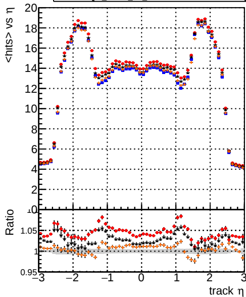
mean hit DOM_mkFit_TTbase DOM_mkFit_TT_retrainOldFiles125 DOM_mkFit_TT_retrainNewFiles125 DOM_mkFit_TT_retrainNewFiles125AndSQCD
