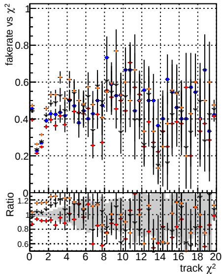
Fake rate vs. BQM mkFit Ttbase BQM mkFit Ttbase+oldFiles125 BQM mkFit Ttbase+newFiles125 AndSQCD
