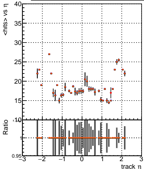
mean hit <math>\langle \text{chits} \rangle \text{ vs } \eta</math>
