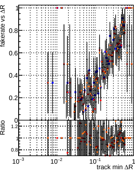
Fake rate vs \Delta R (track, jet) Legend: DOM (black), mktFit (blue), Tbase (red), retrainOldFiles125 (orange), retrainNewFiles125 (green), retrainNewFiles125AndSQCD (purple)
