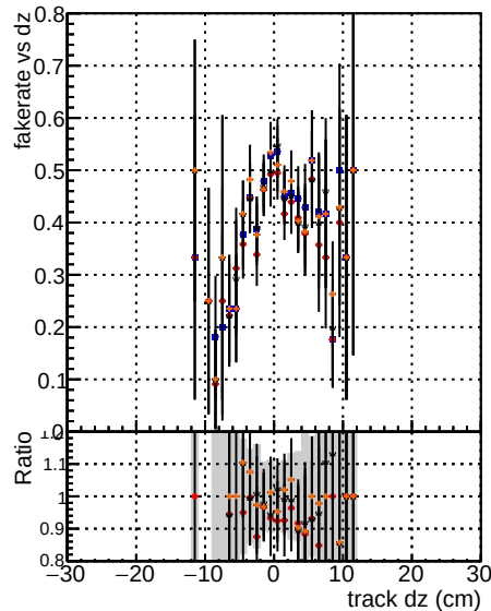
Fake rate vs dz Legend: BQM mktFit TTbase BQM mktFit TTbase OldFiles125 BQM mktFit TTbase NewFiles125 AndSQCD
