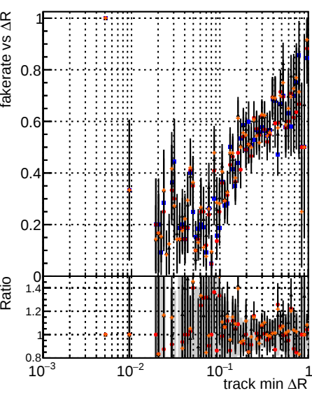
Fake rate vs \Delta R(\text{track, jet}) Legend: DOM mkFit TTbase DOM mkFit retrainOldFiles125 DOM mkFit retrainNewFiles125 DOM mkFit retrainNewFiles125AndSQCD
