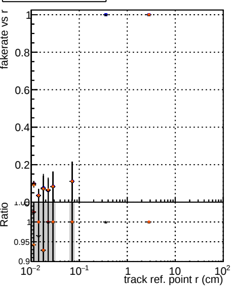
Fake rate vs v DOM mktFit Tbase retrainOldFiles125 retrainNewFiles125 retrainNewFiles125AndSQCD
