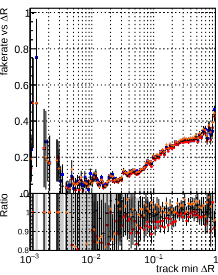
Fake rate vs \Delta R (track, jet) for DOM, mktFit, retrainOldFiles125, retrainNewFiles125, and retrainNewFiles125AndSQCD
