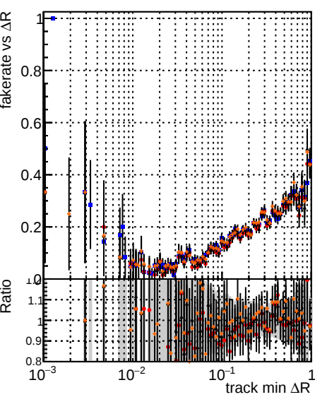
Fake rate vs \Delta R (track, jet) for DOM, mktFit, Tbase, retrainOldFiles125, retrainNewFiles125, and retrainNewFiles125AndSQCD
