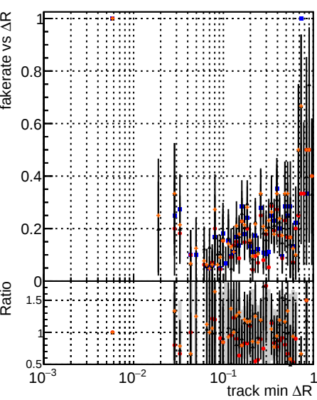
Fake rate vs ΔR(track, jet) Legend: DOM mktFit Tbase retrainOldFiles125 DOM mktFit Tbase retrainNewFiles125 DOM mktFit Tbase retrainNewFiles125AndSQCD
