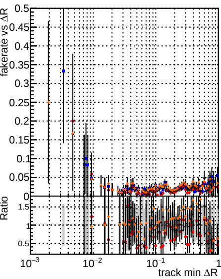
Fake rate vs \Delta R(\text{track, jet}) Series Color Shape base Black Line retrainOldFiles125 Blue Circle retrainNewFiles125 Red Triangle retrainNewFiles125AndSQCD Orange Star
