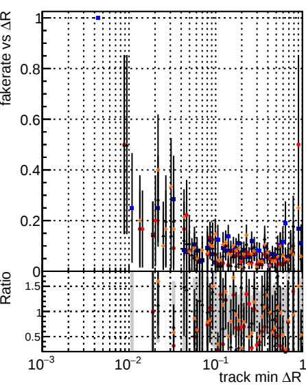
Fake rate vs \Delta R(\text{track, jet}) Legend: DOM (black) mktFit (blue) Tbase (red) retrainOldFiles125 (orange) retrainNewFiles125 (green) retrainNewFiles125AndSQCD (purple)
