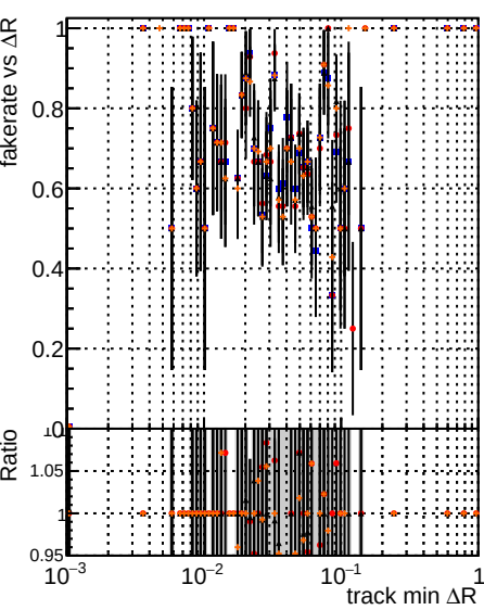
Fake rate vs \Delta R(\text{track, jet}) Legend: DOM (black) mkFit (blue) Tbase (red) retrainOldFiles125 (green) retrainNewFiles125 (orange) retrainNewFiles125AndSQCD (purple)
