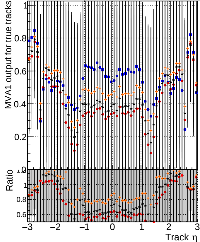
MVA1 of associated tracks (recoToSim) vs. track \eta Legend: DQM_mkFit_TTbase (blue squares) DQM_mkFit_TT_retrainOldFiles125 (red circles) DQM_mkFit_TT_retrainNewFiles125 (black stars) DQM_mkFit_TT_retrainNewFiles125AndSQCD (orange crosses)
