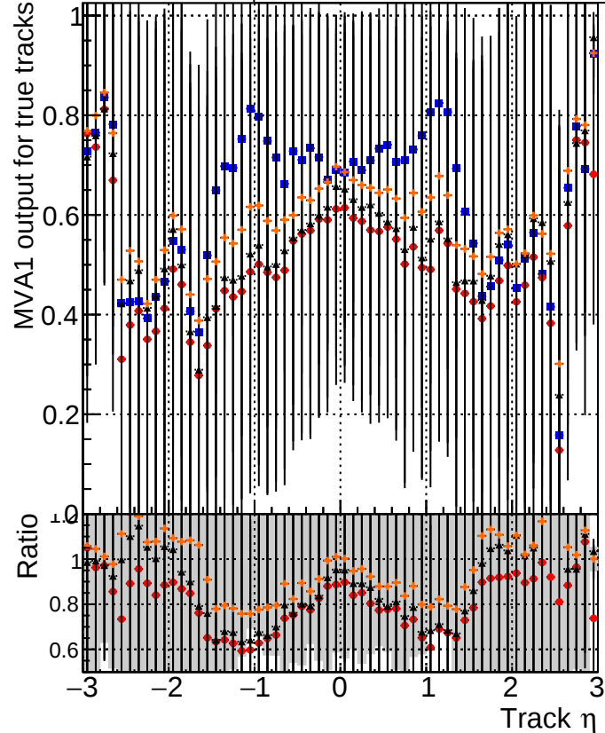
MVA1 of associated tracks (recoToSim) vs. track \eta Legend: DQM_mkFit_TTbase (blue squares) DQM_mkFit_TT_retrainOldFiles125 (red diamonds) DQM_mkFit_TT_retrainNewFiles125 (black stars) DQM_mkFit_TT_retrainNewFiles125AndSQCD (orange crosses)
