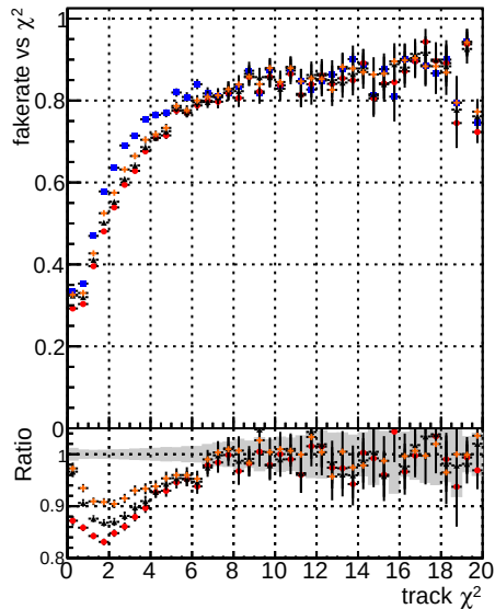
Fake rate vs. \chi^2 Legend: BQM mkFit TTbase Ttbase Ratio: Ratio of fake rate to seed rate
