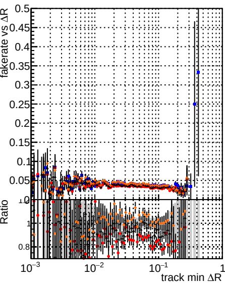
Fake rate vs \Delta R (track, jet) DOM mkFit TTbase DOM mkFit retrainOldFiles125 DOM mkFit retrainNewFiles125 DOM mkFit retrainNewFiles125AndSQCD
