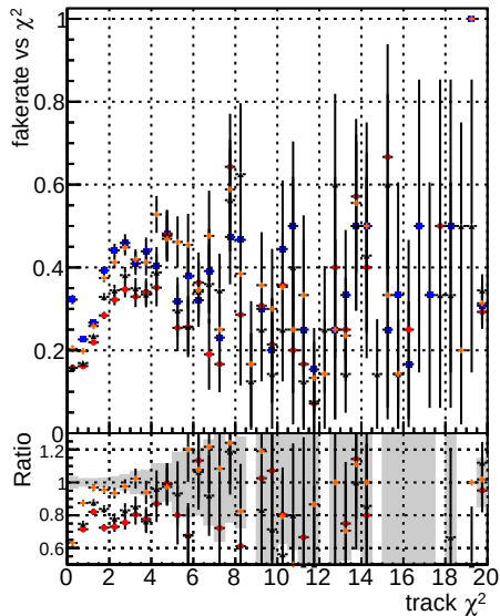
Fake rate vs. BQM mkFit TTbase BQM mkFit TTbase TrainOldFiles125 BQM mkFit TTbase TrainNewFiles125 AndSQCD
