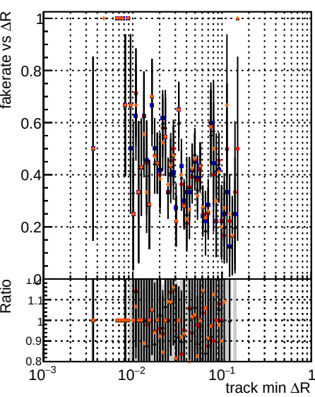
Fake rate vs \Delta R(\text{track, jet}) DOM mkFit + base DOM mkFit + retrainOldFiles125 DOM mkFit + retrainNewFiles125 DOM mkFit + retrainNewFiles125AndSQCD
