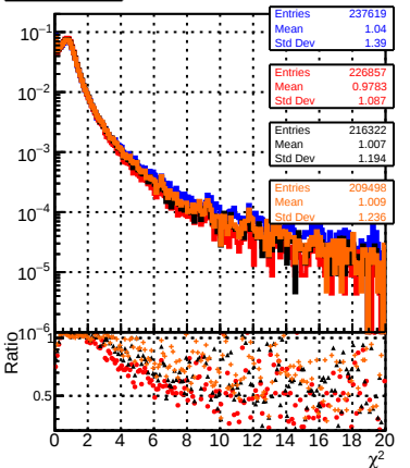
normalized \chi^2
