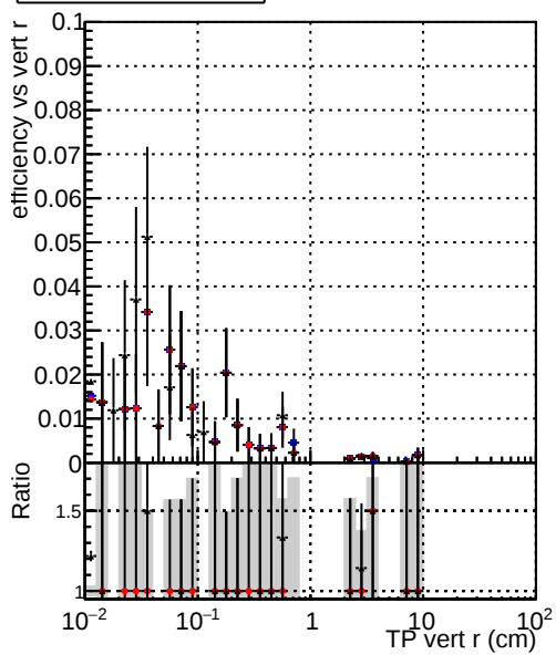
Efficiency vs verpos
